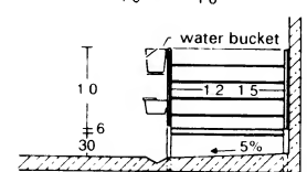
6 Single stalls for calves (14 days to 10 weeks)
